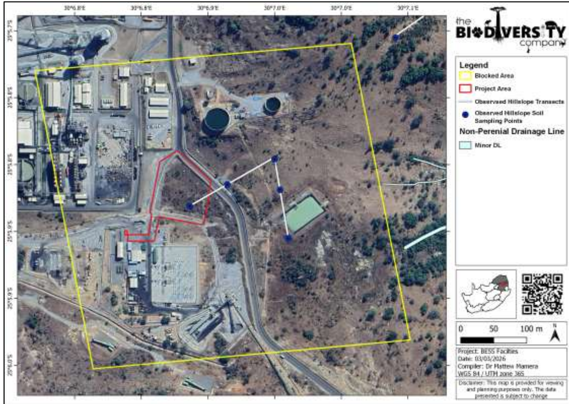
Figure 1 The identified drainage lines in relation to the proposed BN BESS Project.
