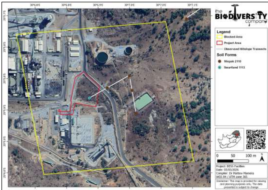
Figure 2 The assessed hillslope transects hydrogeological patterns regarding the BN BESS Project
